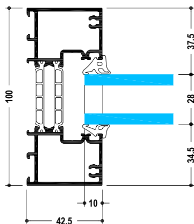
Pocket framing for glass up to 32 mm
