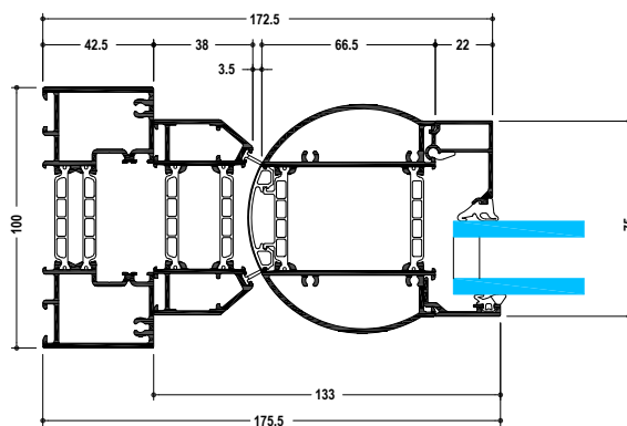
Anti-finger trap safety stile
