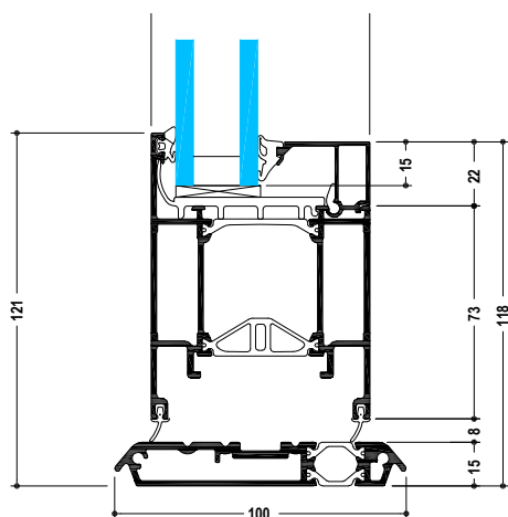
Low threshold 15 mm
