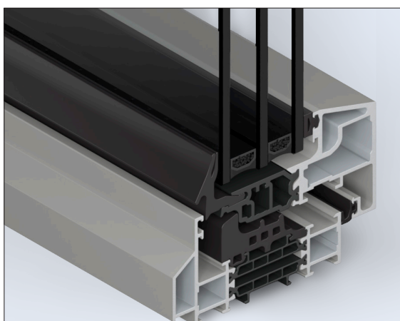
SOLEAL NEXT 75 Minimal Slope frame and Slope vent
