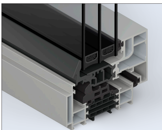
SOLEAL NEXT 75 Minimal Step frame and Square vent
