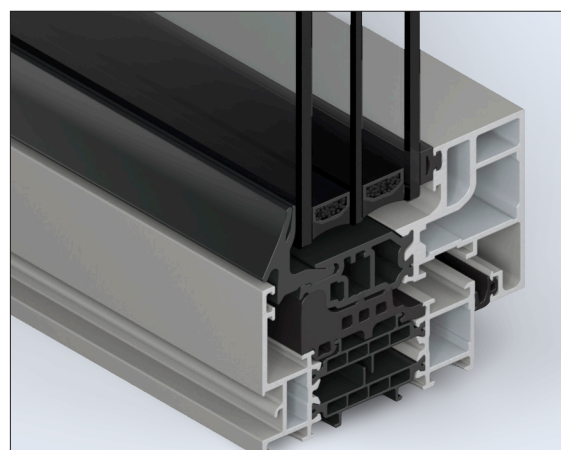
SOLEAL NEXT 75 Minimal Concealed drainage frame and Square vent
