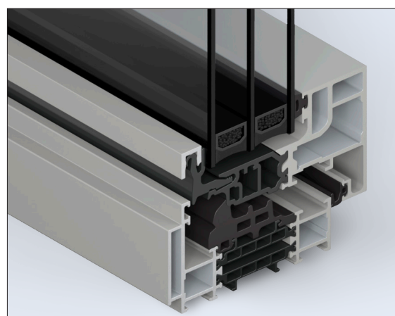
SOLEAL NEXT 75 Minimal Clip-On-Trim Step frame and Square vent
