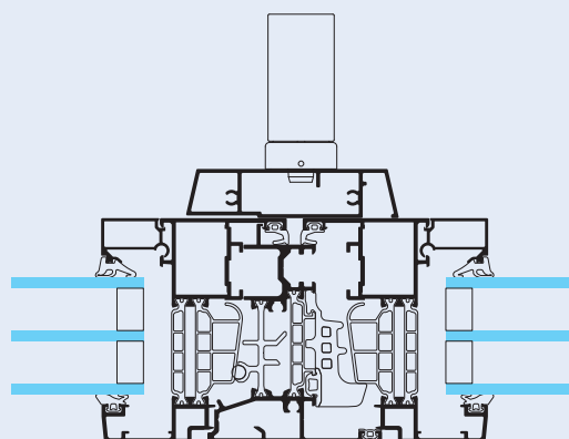
SOLEAL NEXT Visible centered handle
